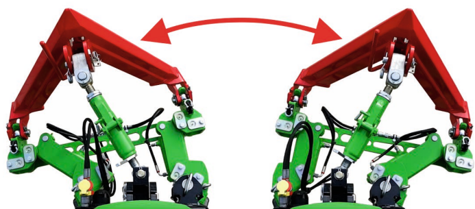
Sauter swivel lower links-for even more flexibility of the front implement
